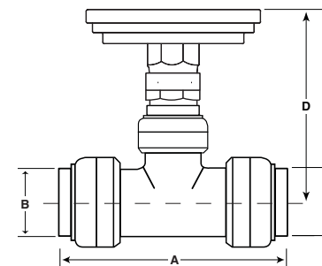
Temperature Gauge with Fittings Dimensions
